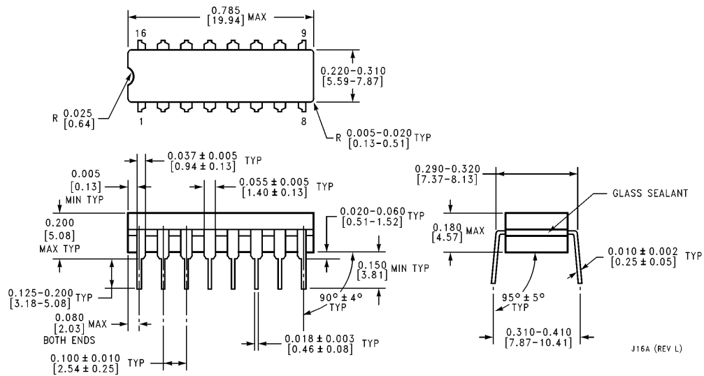
16-Lead Ceramic Dual-In-Line Package (J) Order Number DM54145J NS Package Number J16A
