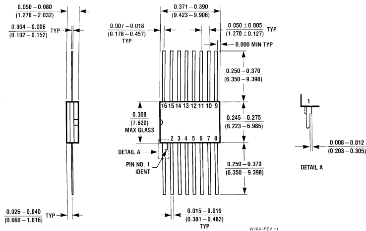
16-Lead Ceramic Flat Package (W) Order Number DM54145W NS Package Number W16A
